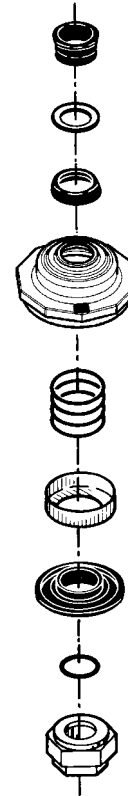
Fig. 11 Shaft seal, MS 4000
